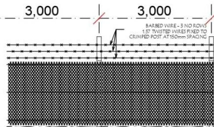
TYPICAL ELEVATION
