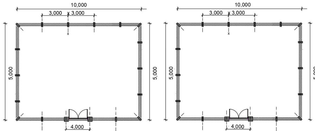
GROUND LAYOUT PLAN
