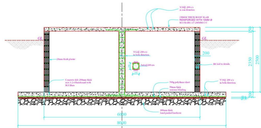
SECTION X-X
