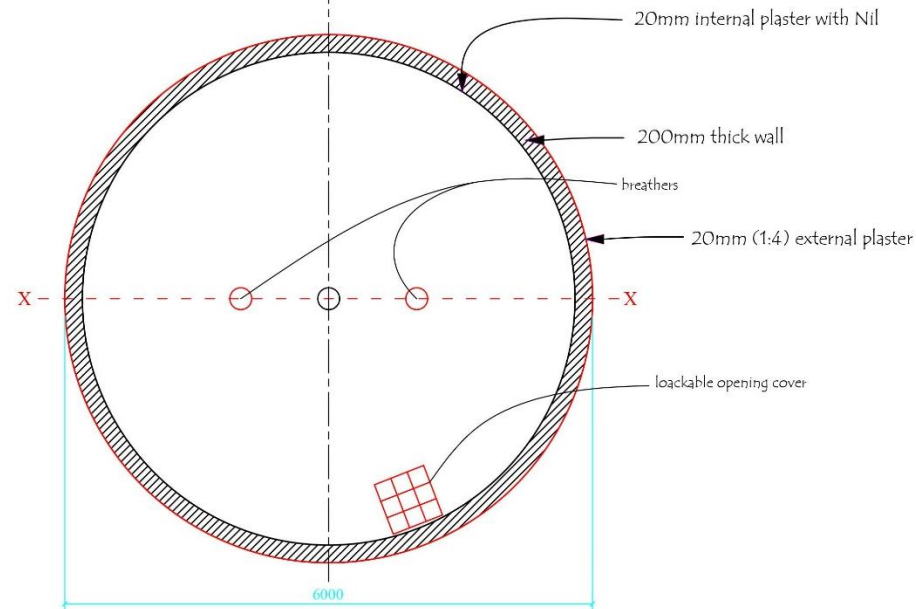
PLAN Scale 1:50
