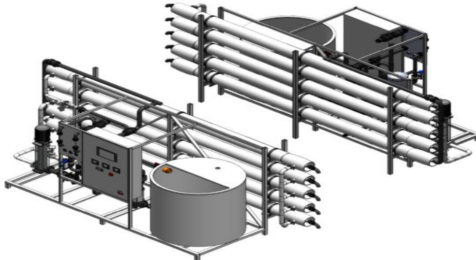
Reverse Osmosis Plant Layout.
