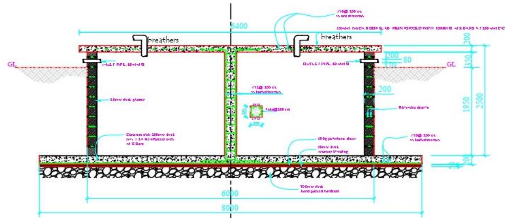
SECTION X-X
