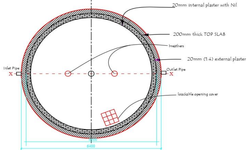
PLAN Scale 1:50
